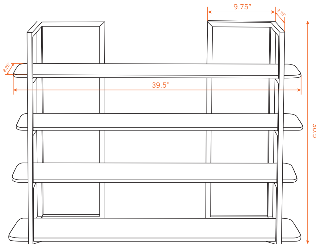
HI-RISE CORNERS
